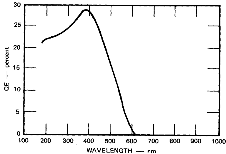
FIGURE 2 (U) SPECTRAL RESPONSE OF 9829 QB PM TUBE
